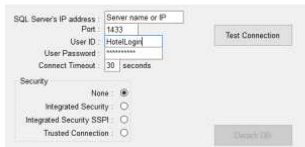
(Picture 5, parameters for connecting to SQL Server)
